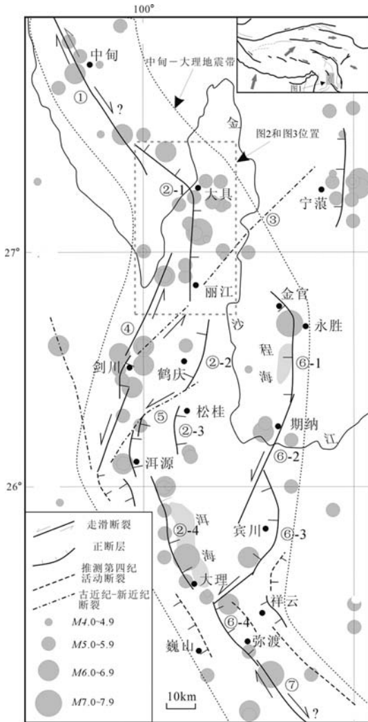
图1 滇西北裂陷带区域构造简图 ① Fig. 1 Regional tectonic map of Northwestern Yunnan Rift Zone
