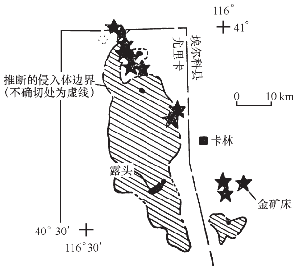
图4 卡林矿床附近与金矿有关的花岗岩的分布 [8] Fig.4 Distribution of granite related to gold deposits in the vicinity of the Carlin-type deposit
